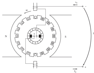
Figure 7-28 A dc machine with interpoles.
